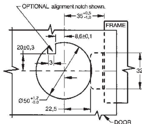
Panel Preparation
