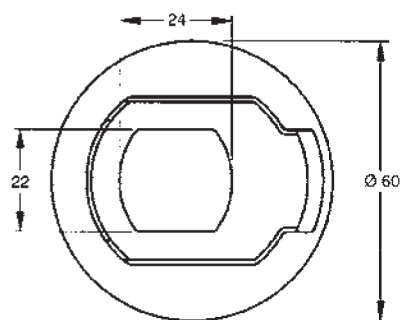
LATCH
