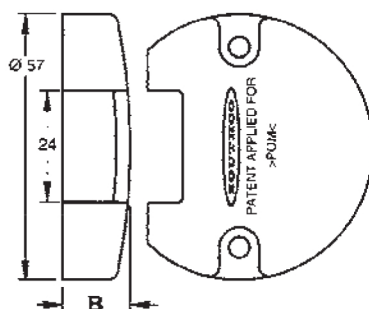
MOUNTING CUP
