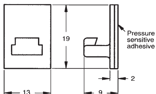
KEEPER ASSEMBLY
