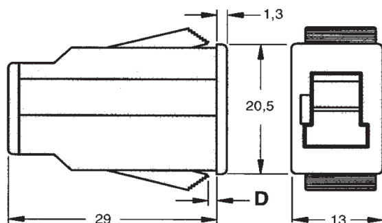
LATCH
