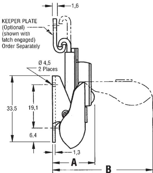
Latch in closed position
