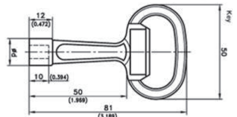
Female (Hollow)
