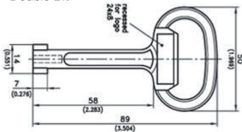
Double Bit
