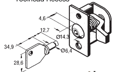
Toolhead Recess
