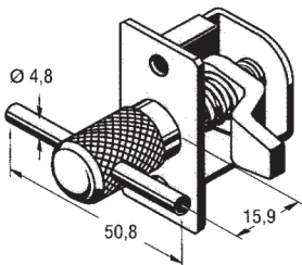
Knurled Head with T-bar
