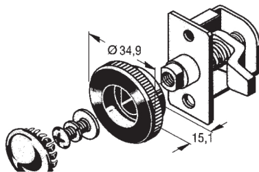
Head-Socket
