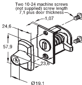
Keylocking
