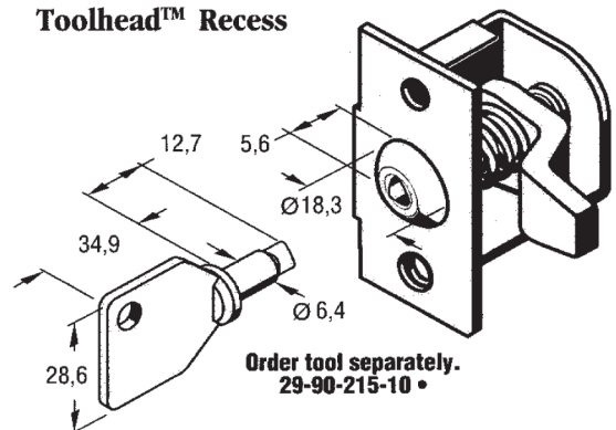
Toolhead™ Recess
