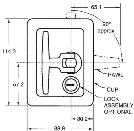
TYPE A Assembly Illustrated
