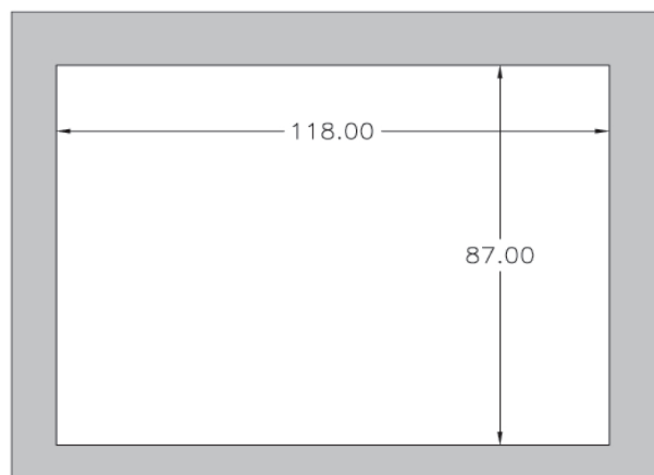
PANEL CUT-OUT
