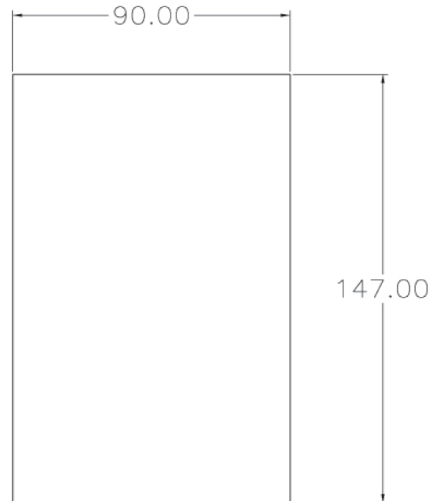
PANEL CUT-OUT
