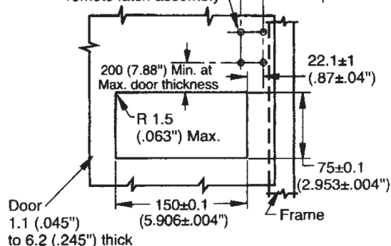
Mounting hole pattern for remote latch assembly
