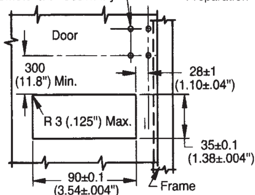
Mounting hole pattern for remote latch assembly
