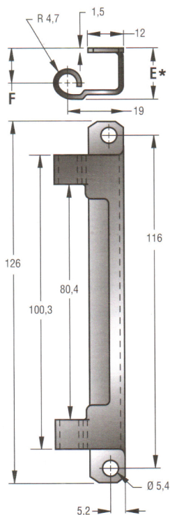
Frame Leaf
