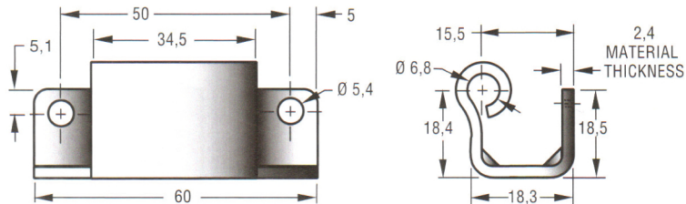
Formed Frame Leaf (P/N: F6-905-5)
