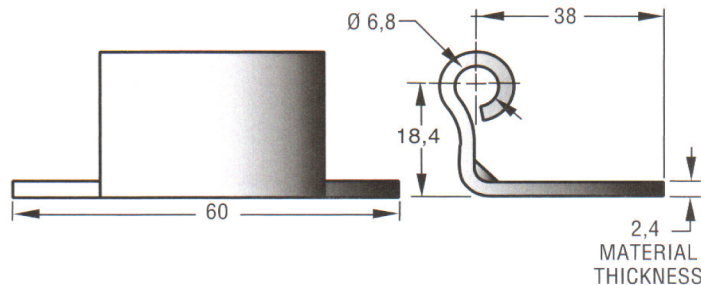
Formed Frame Leaf (P/N: F6-904-5)
