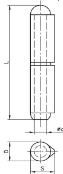
Version B with loose pin
