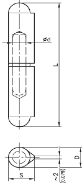
Version A with fixed pin
