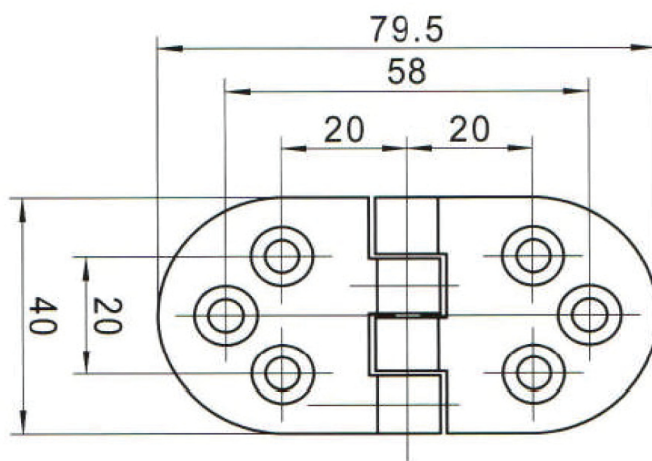
P/N: SCL-238-3 Material: Stainless steel
