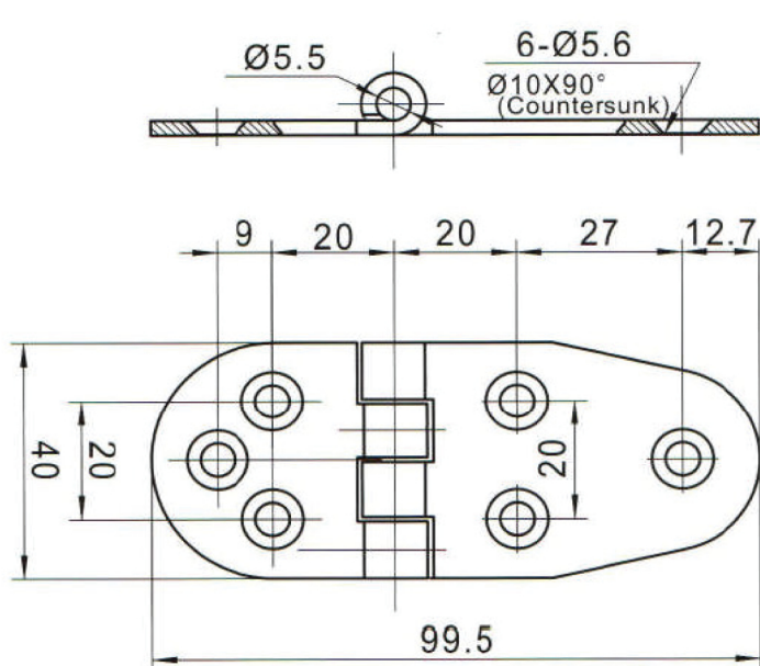
P/N: SCL-238-1 Material: Stainless steel
