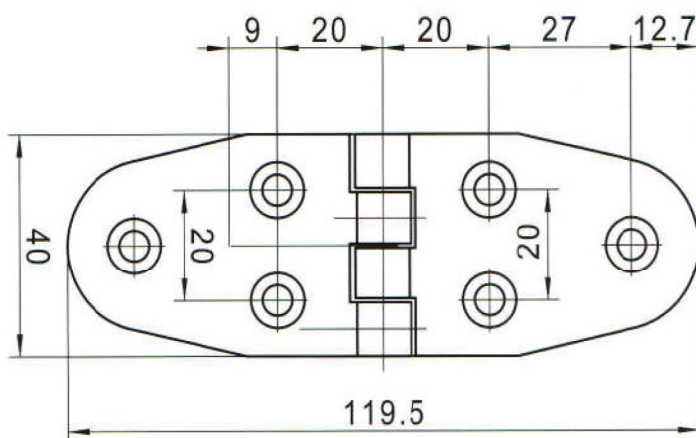
P/N: SCL-238-2 Material: Stainless steel
