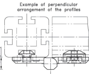
Fastening/Positioning blocks for application with non DIRAK tenon blocks
