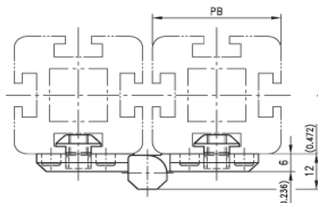
Tenon blocks for positioning and fastening
