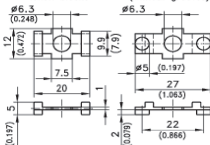
Fastening/Positioning blocks for application with non DIRAK tenon blocks
