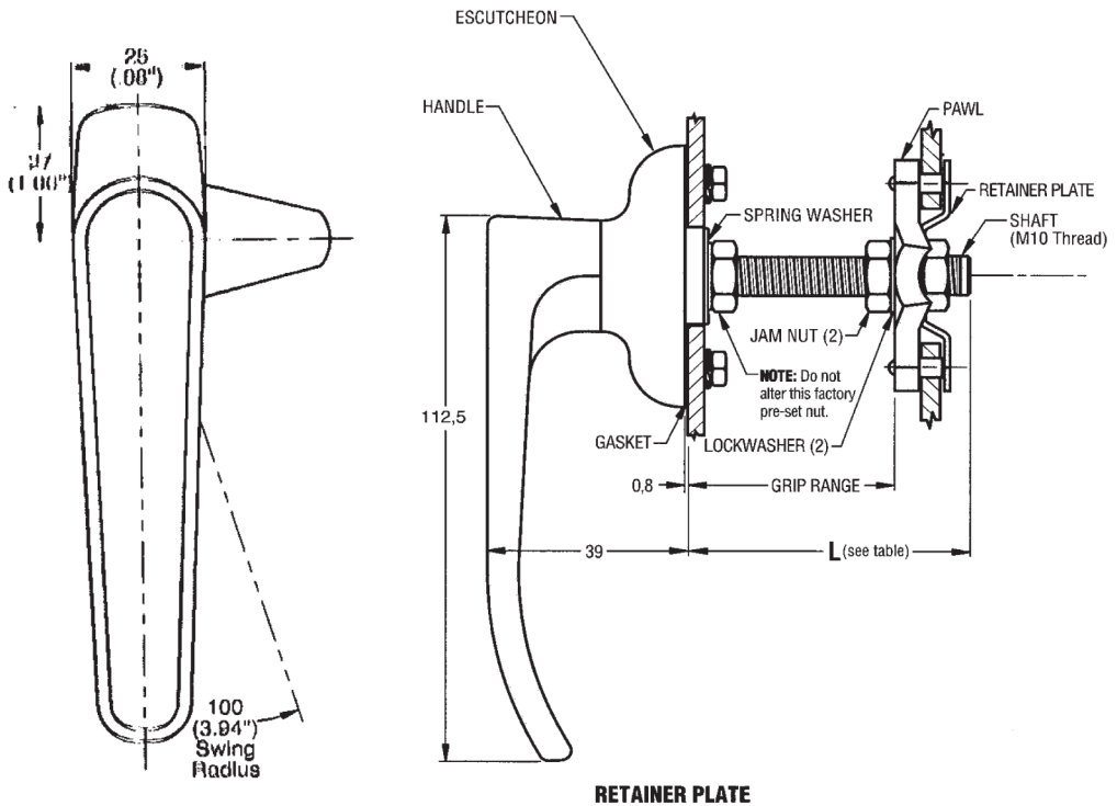
RETAINER PLATE
