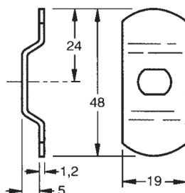
RETAINER PLATE
