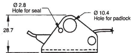
Latch body with features for tamper resistant
