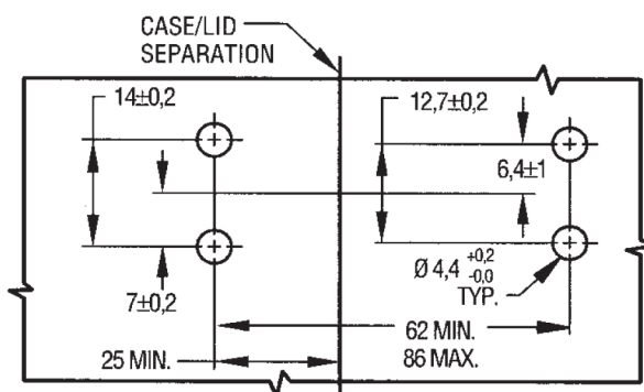
Exposed Base Latch - Exposed keeper
