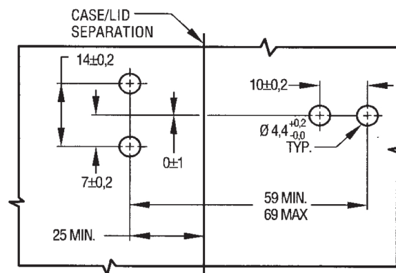
Exposed Base Latch - Concealed keeper
