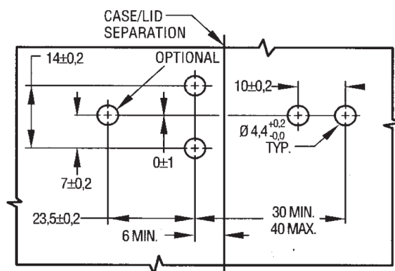
Concealed Base Latch - Concealed keeper
