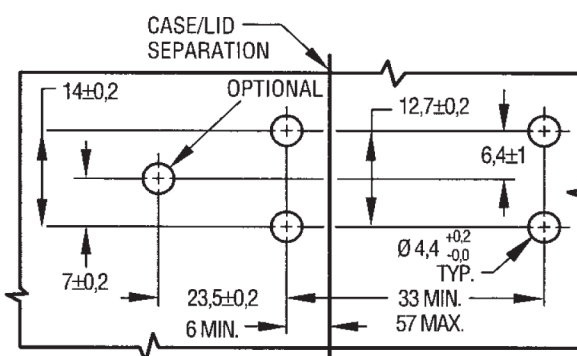
Concealed Base Latch - Exposed keeper
