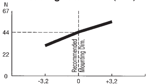
Steady state clamp force vs. mounting dimension (21°C)
