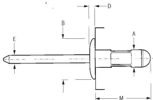
BEFORE PLACING
