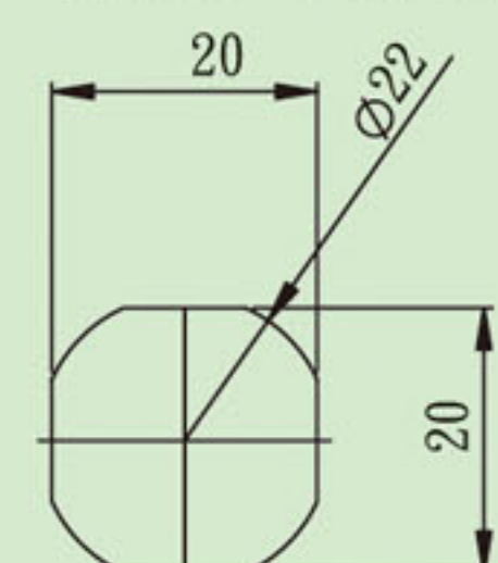
PANEL CUTOUT DIMENSION
