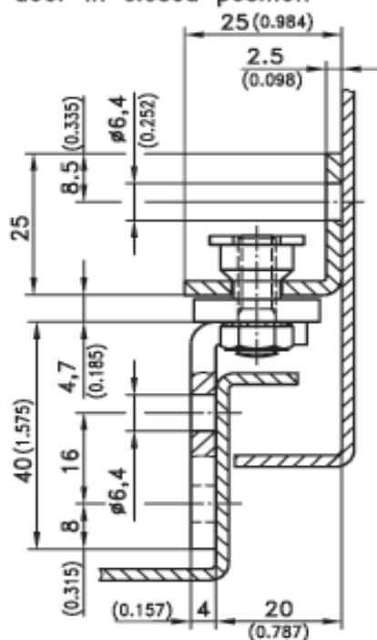
view A-B door in closed position
