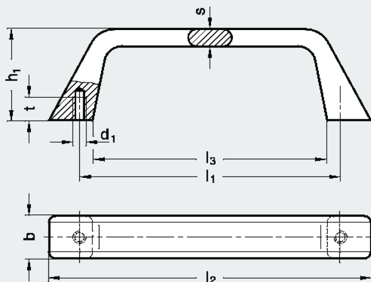
Type A mounting from the back
